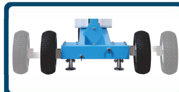
Wheel base adjustable from 80cm to 140 cm for better stability.
